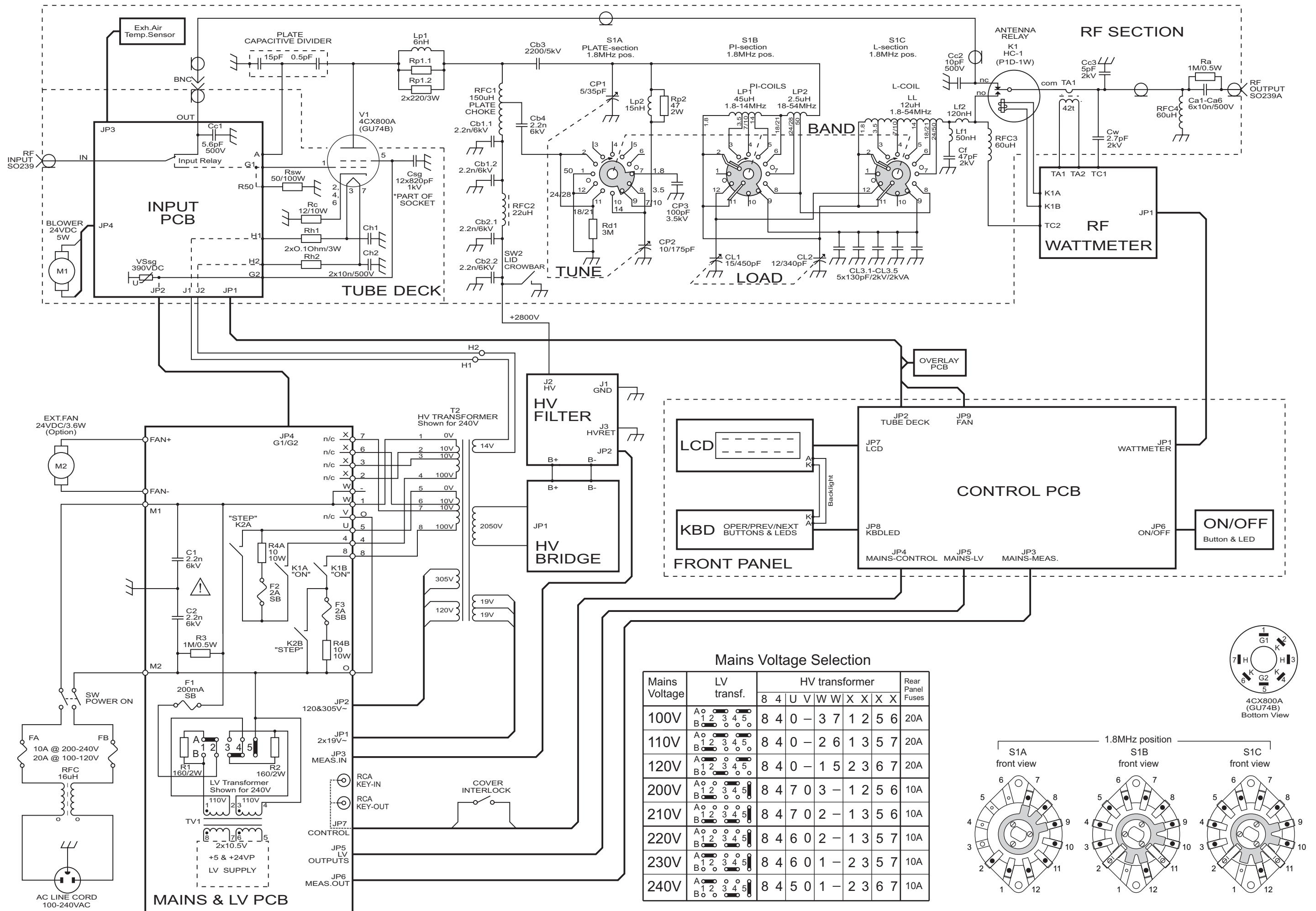
Fig. 6.1 ACOM1000 Simplified Schematic Diagram
